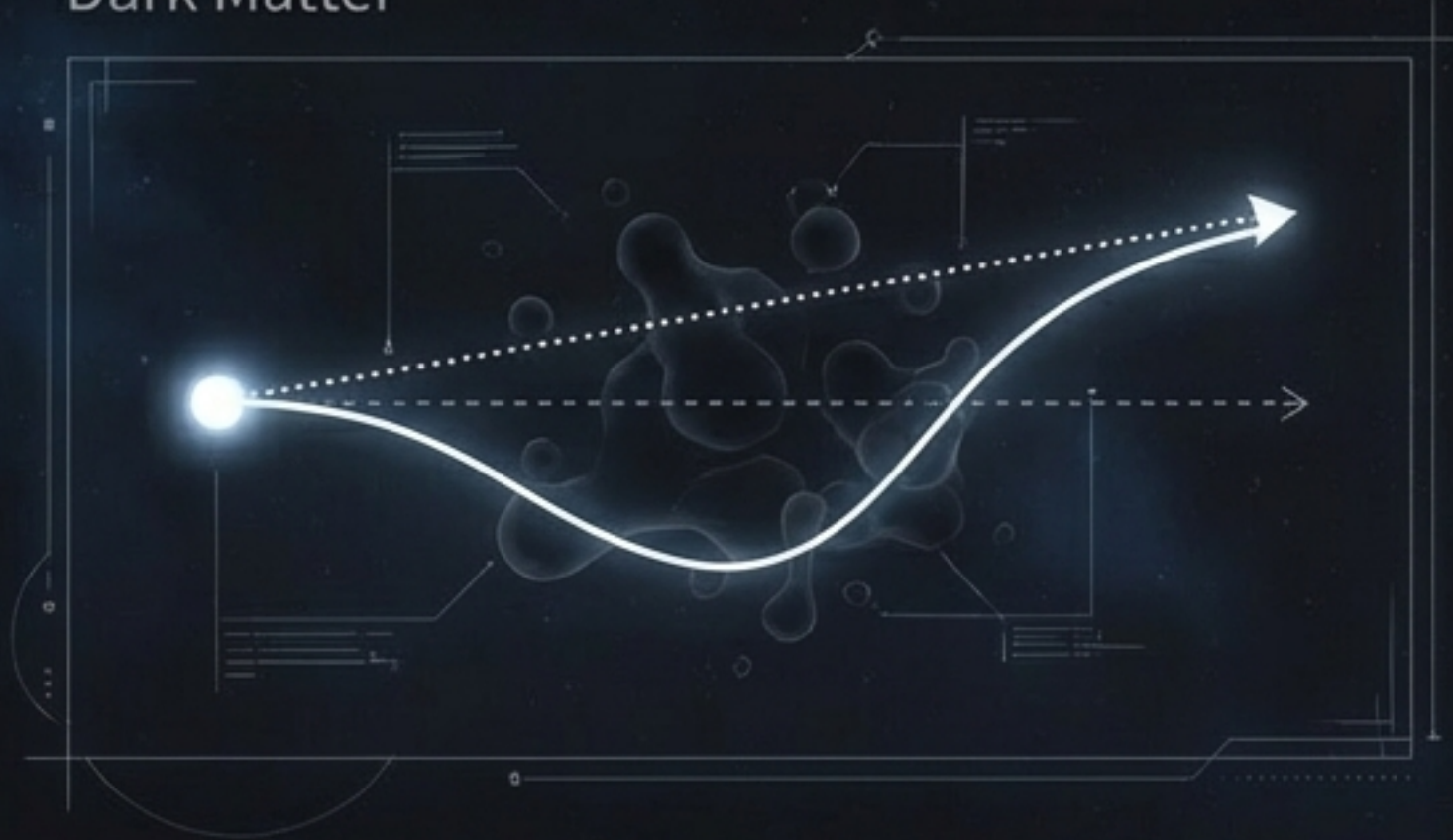
Dark Matter
